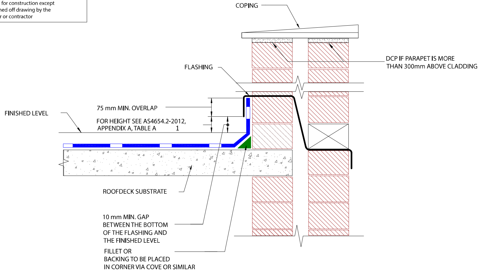
CAVITY WALL DETAIL
